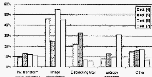
Fig. 1. Time breakdown of an H.264/AVC decoder on General Purpose Processors as reported in [4]-[7]
